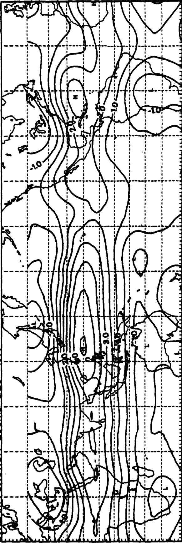
STREAM FUNCTION 200MB DEC 1977
